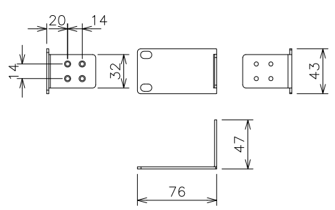
Mounting bracket (for 19-inch rack)
