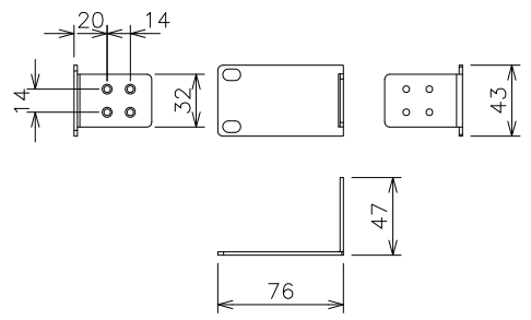
Mounting bracket (for 19-inch rack)
