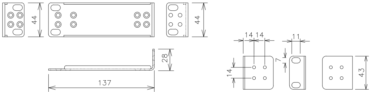
Mounting bracket (for 19-inch rack)
