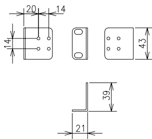
Mounting bracket (for 19-inch rack)
