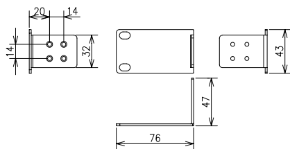
Mounting bracket (for 19-inch rack)
