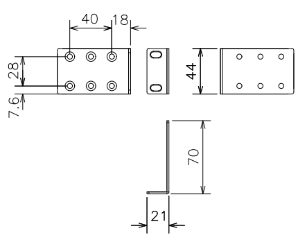
Mounting bracket(for 19-inch rack)
