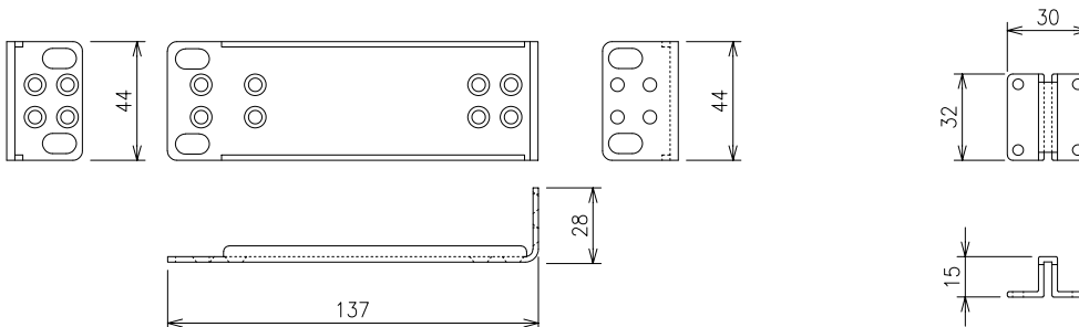
Mounting bracket (for 19-inch rack)
