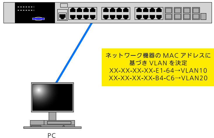
図 61-1 Static MAC-based Subnet VLAN の概略
