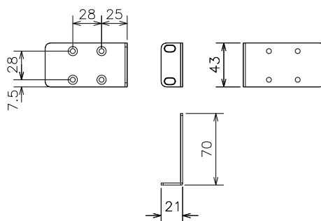
Mounting bracket (for 19-inch rack)
