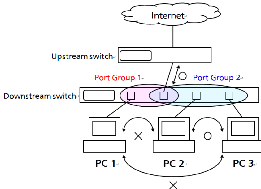
Figure 3-42 Example of Configuration Using Port Grouping
