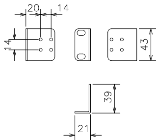
Mounting bracket (for 19-inch rack)
