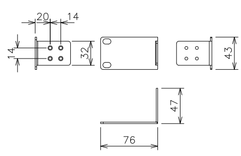
Mounting bracket (for 19-inch rack)
