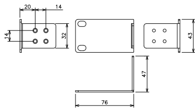
Mounting bracket(for 19-inch rack)
