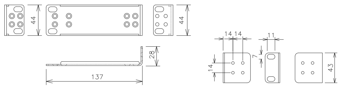
Mounting bracket (for 19-inch rack)
