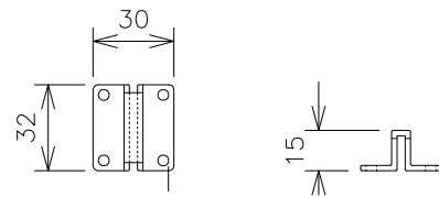
Connecting bracket
