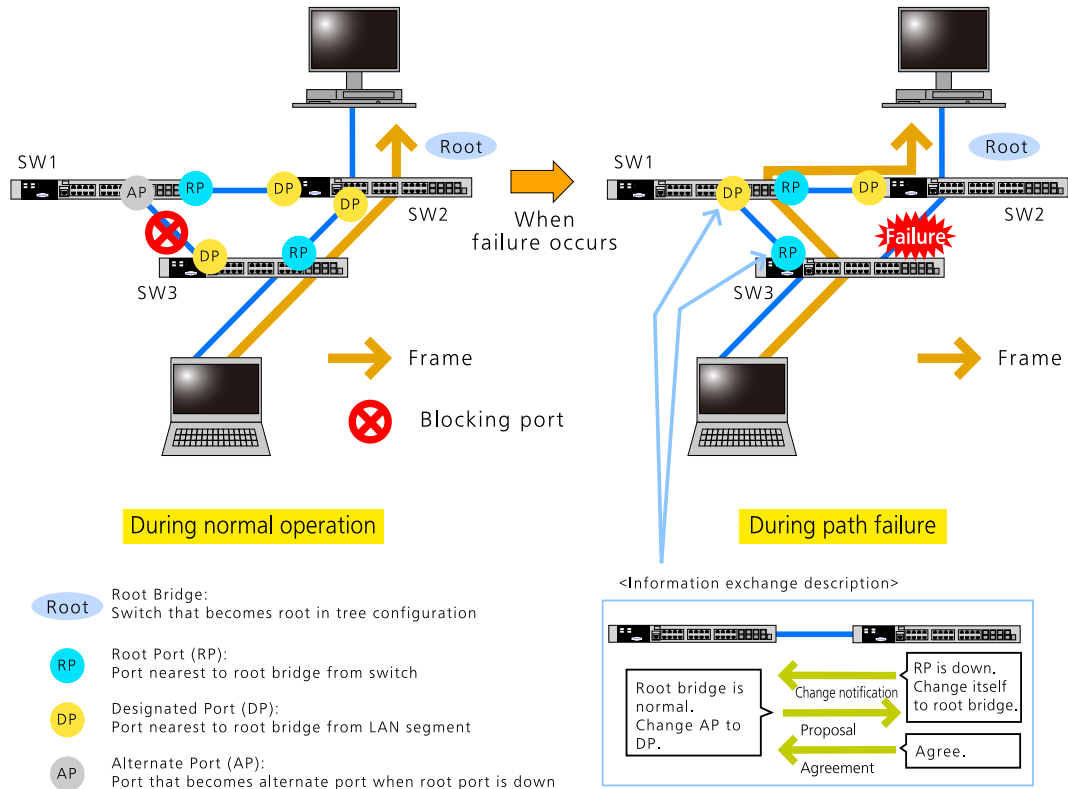
Figure 71-2 RSTP overview
