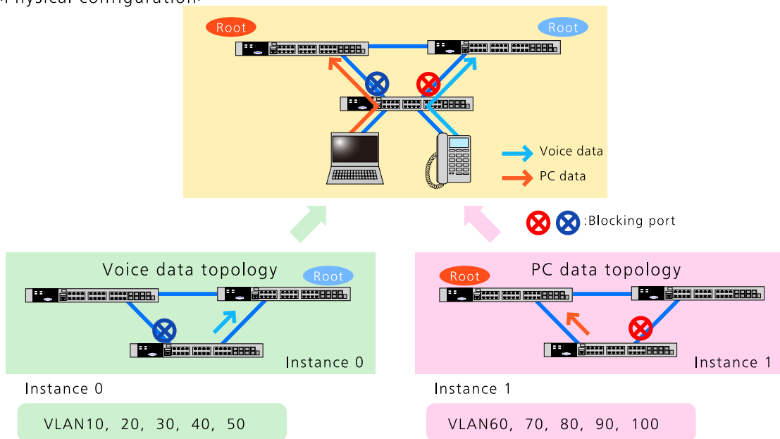
Figure 71-3 MSTP overview
