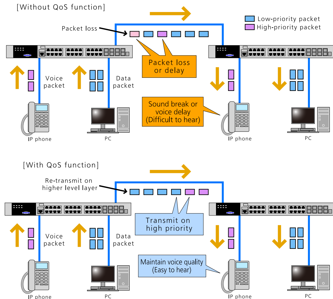
Figure 41-1 QoS overview
