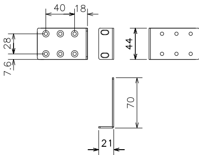
Mounting bracket(for 19-inch rack)
