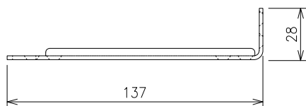
Mounting bracket (for 19-inch rack)
