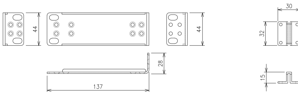
Mounting bracket (for 19-inch rack)
