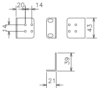
Mounting bracket
