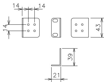
Mounting bracket (for wall mount)
