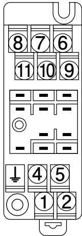
SOCKET TOP VIEW
