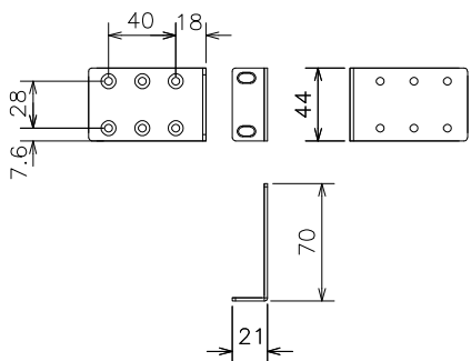
Mounting bracket(for 19-inch rack)
