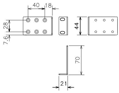
Mounting bracket(for 19-inch rack)
